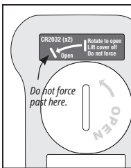
Battery Cover
